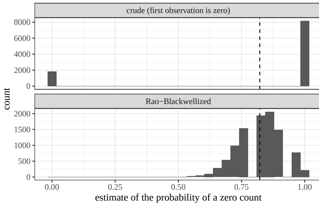
Figure 1: The sampling distribution of the crude and Rao–Blackwellized estimators ( n = 20, 10,000 samples); the dashed line marks the estimand
