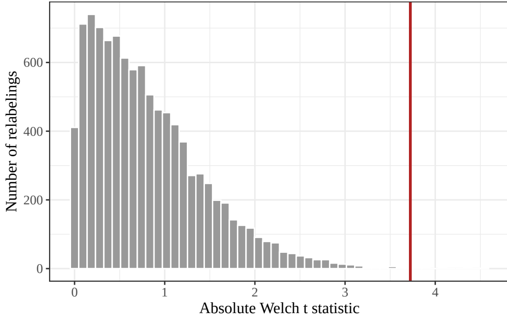
Figure 1: Permutation distribution of the absolute Welch t statistic for gene 3, from 10,000 random relabelings of tumor classes 2 and 4. The vertical line is the observed statistic.
