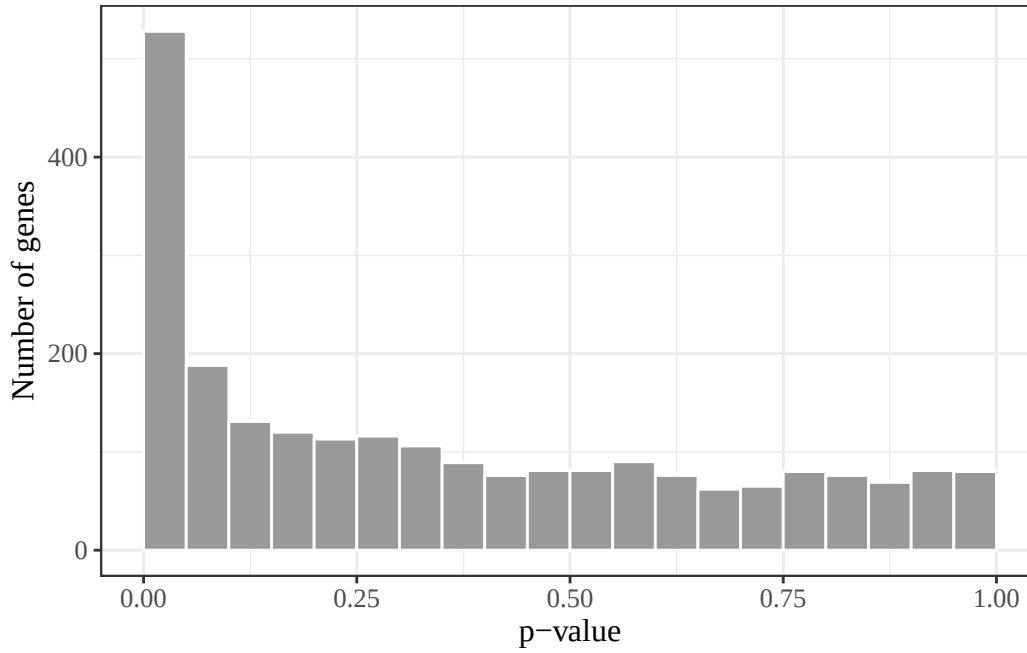
Figure 1: Histogram of the 2308 Welch t-test p-values comparing tumor classes 2 and 4 in the Khan data.
