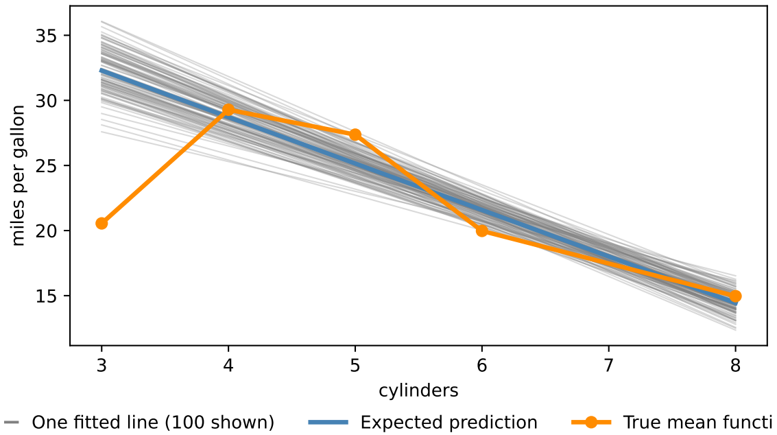
Figure 1: The fitted lines of 100 of the 2000 training sets (grey), their pointwise expected prediction (blue), and the true mean function (orange), for mpg against cylinders .
