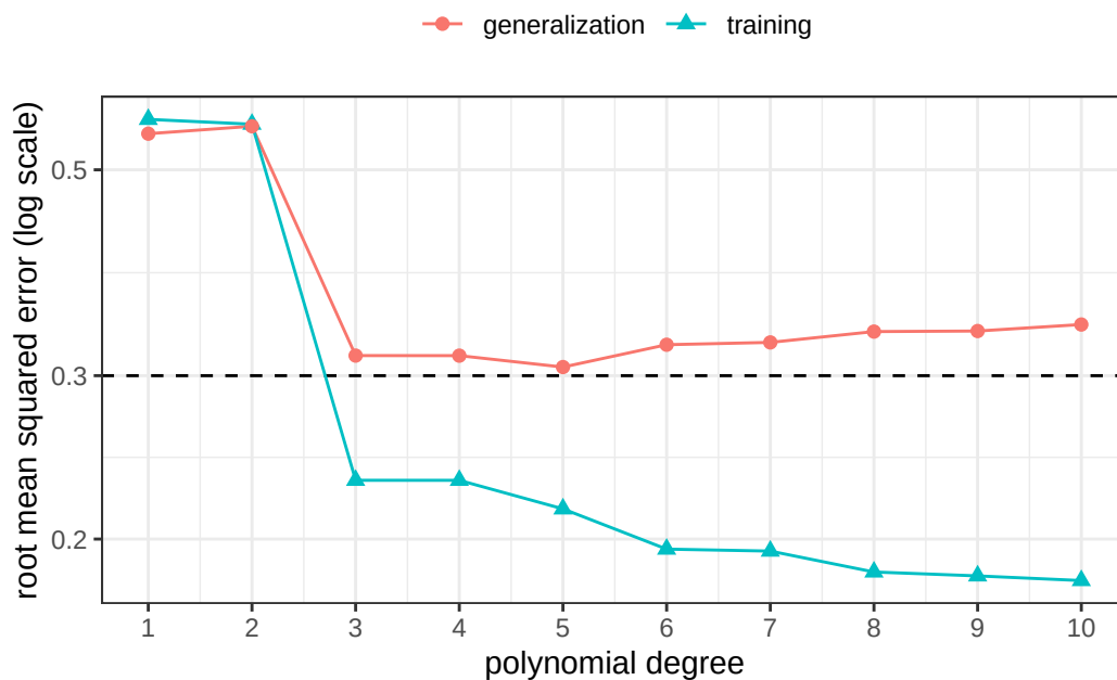
Figure 2: Training sRMSE and estimated generalization error (sRMSE on 10,000 new observations) of polynomial fits to one simulated training set of n = 30 . The dashed line is the noise standard deviation \sigma , the square root of the residual variance .
