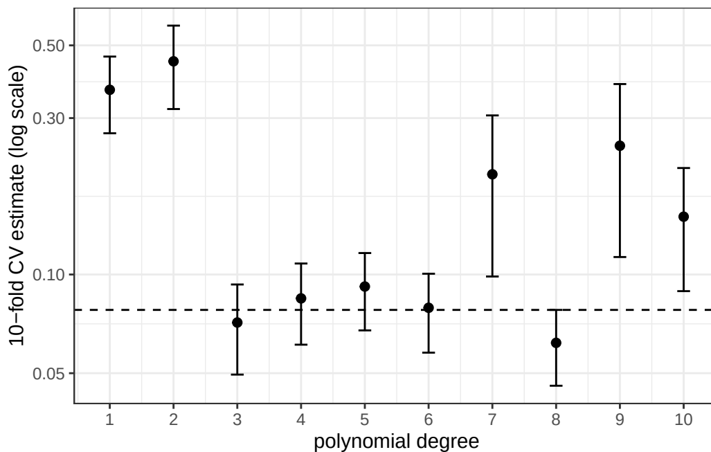
Figure 8: 10-fold cross-validation estimates, with bars of one fold-based standard error (Equation 63). The dashed line is one fold-based standard error above the smallest estimate.
