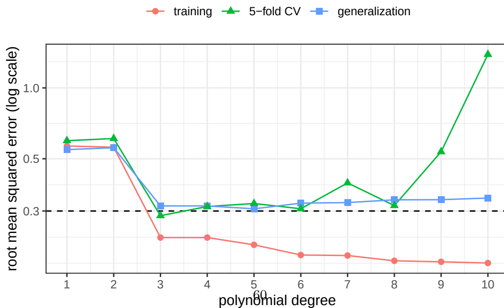
Figure 7: Figure 2 with the 5-fold cross-validation estimate added. Only the training and cross-validation curves could be computed from real data.
