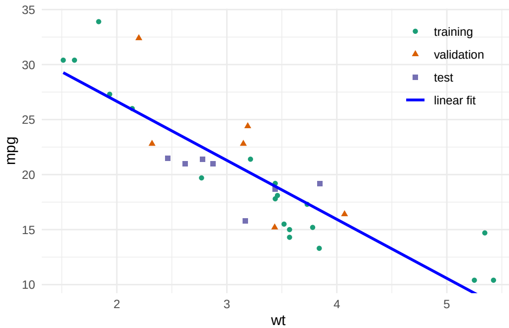
Figure 3: Linear model fit superimposed on data partitions
