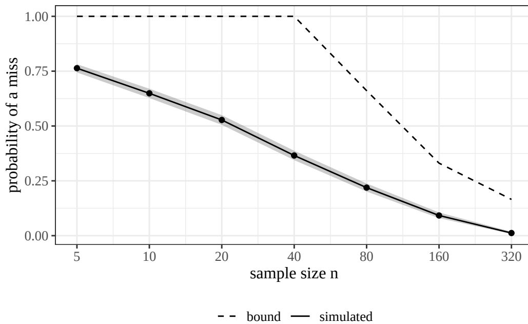
Figure 1: The chance that the sample mean of n birth weights misses the population mean by 100 g or more, by simulation (2000 repeats per n , with 95% confidence bands) and by the bound from Lemma 0.1
