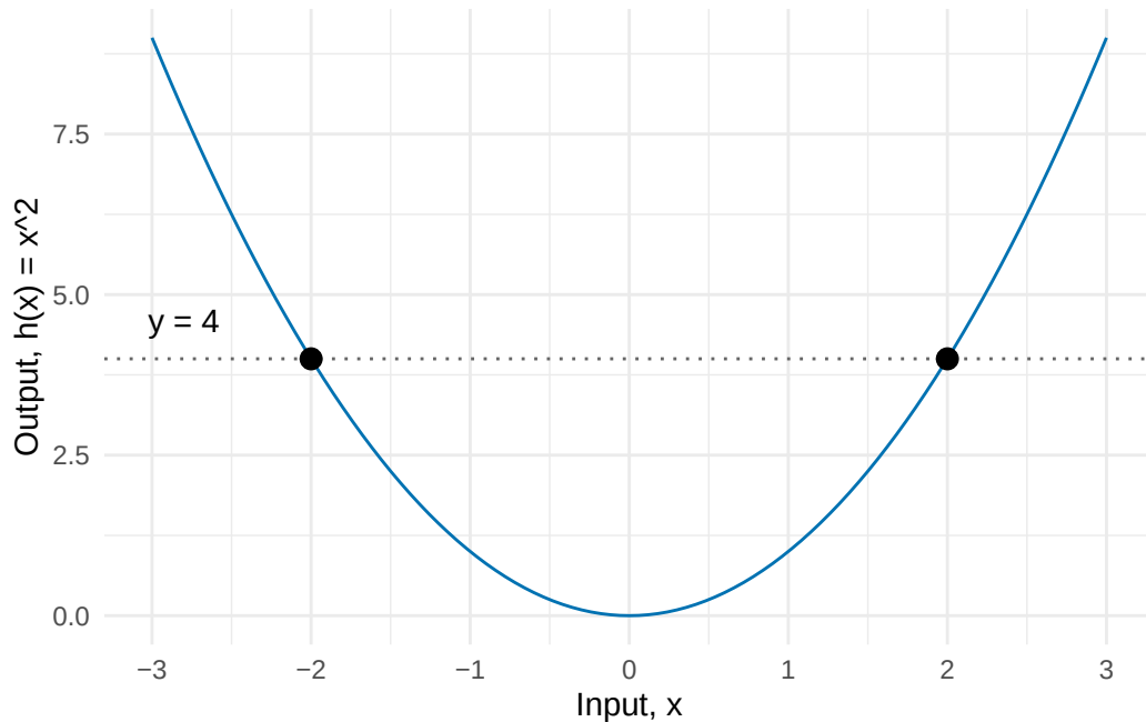
Figure 7: The horizontal line y = 4 meets the 13 graph of h(x) = x^2 twice, at x = -2 and x = 2 , so h has no inverse function .
