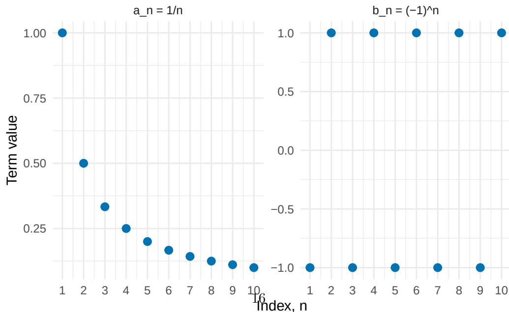
Figure 8: The first ten terms of the sequences a_n = 1/n and b_n = (-1)^n of Example 0.14, plotted against n . The terms of b_n take only two values.
