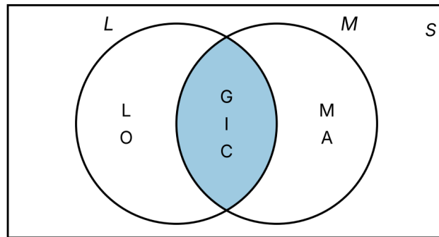
Figure 1: The letters of LOGIC ( L ) and of MAGIC ( M ), with L \cap M shaded.
