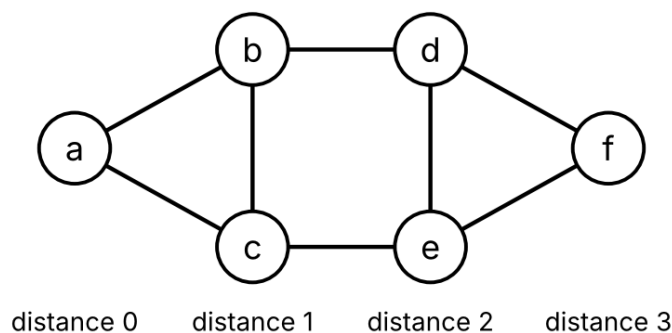
Figure 9: The office graph, with its vertices in columns by their distance from a .
