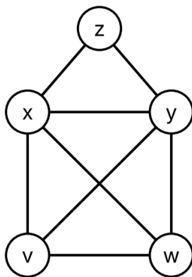
Figure 8: An envelope: a square with both diagonals and a roof.
