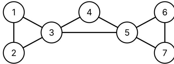
Figure 6: The graph T : three triangles in a row.
