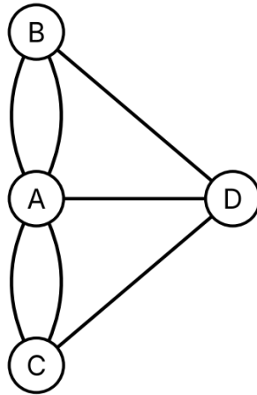
Figure 3: The bridges of Königsberg as a graph: a vertex for each piece of land, and an edge for each bridge.
