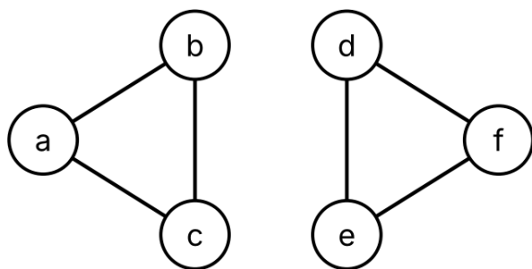
Figure 7: The graph H : the office graph without the edges \{b, d\} and \{c, e\} .
