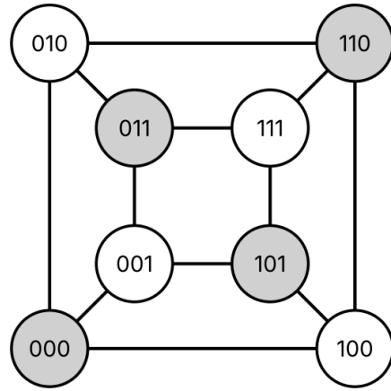
Figure 5: The cube graph Q_3 , with the strings in V_1 shaded.
