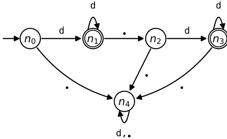
Figure 5: A DFA whose language is the set of numerals.
