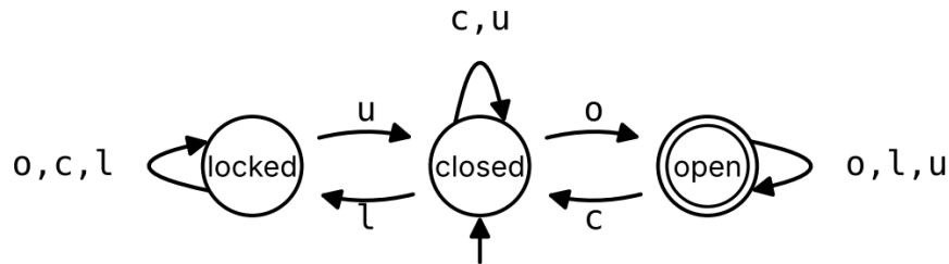
Figure 3: The door as a DFA whose one accepting state is open.
