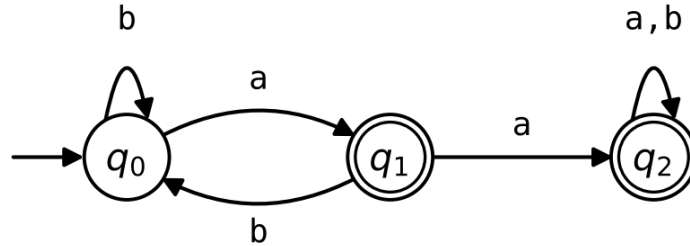
Figure 4: The DFA A' , which accepts the strings that A rejects.
