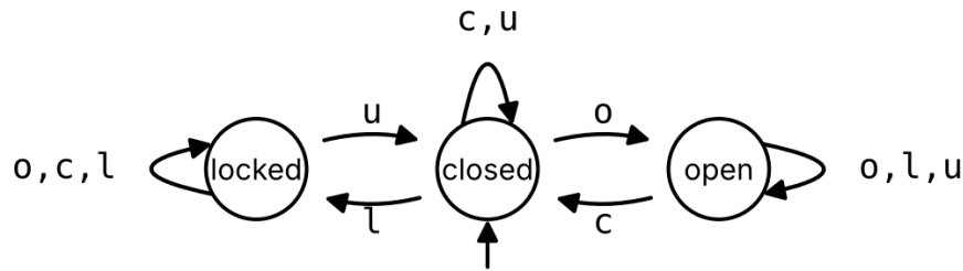
Figure 1: The state diagram of the door.
