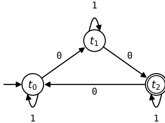
Figure 6: The DFA T , which accepts the strings whose number of 0s leaves remainder 2 when divided by 3.
