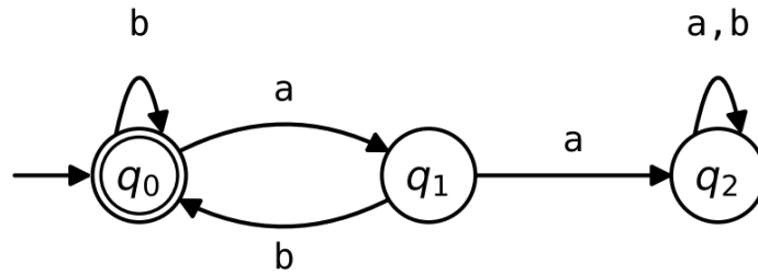
Figure 2: The DFA A , which checks that every a is followed by a b .
