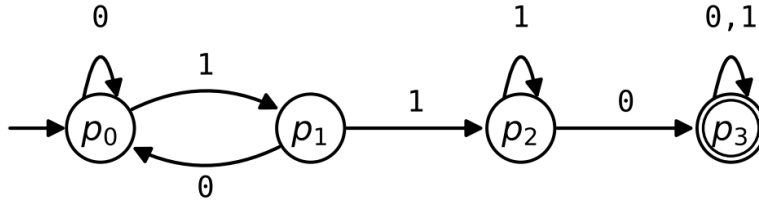
Figure 7: The DFA W , which accepts the strings that contain 110.
